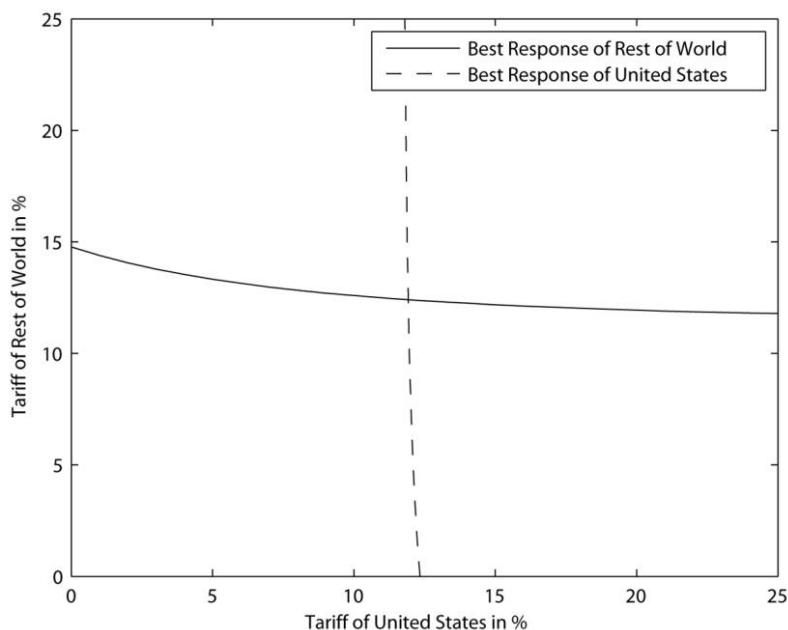
FIG. 2.—Reaction functions and Nash equilibrium
