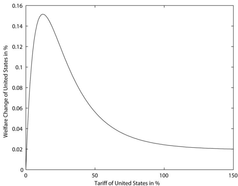
FIG. 1.—Optimal tariff with tariff revenue
