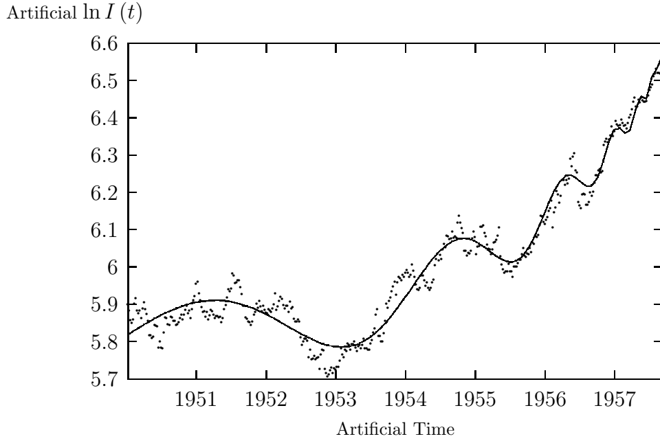
Figure 8: Surrogate data and best fit by equation (22) is A \approx 6.6 , B \approx -.34 , C \approx -.047 , \alpha \approx 0.74 , t_c \approx 1957.7 , \phi \approx -.13 , \omega \approx 9.1 , \Delta_t \approx 4.1 , \Delta\omega \approx -2.1 and r.m.s. \approx 0.037
